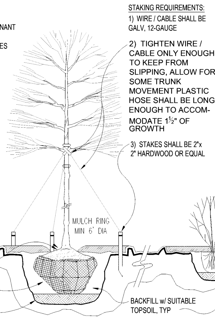
1 PLANTING INSTALLATION DETAILS SCALE: NTS
